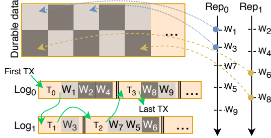
Figure 3: Parallel log replay. The notation W_i denotes a write to address i . \text{Rep}_0 and \text{Rep}_1 are responsible for odd/even addresses respectively.
