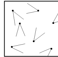
Figure 3: Visibility-based IM
