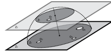
Figure 5: 3-dimensional VFC
