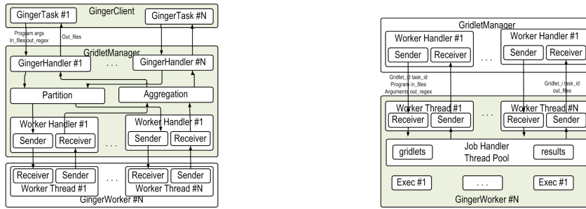
Fig. 2. Gridlet Manager
