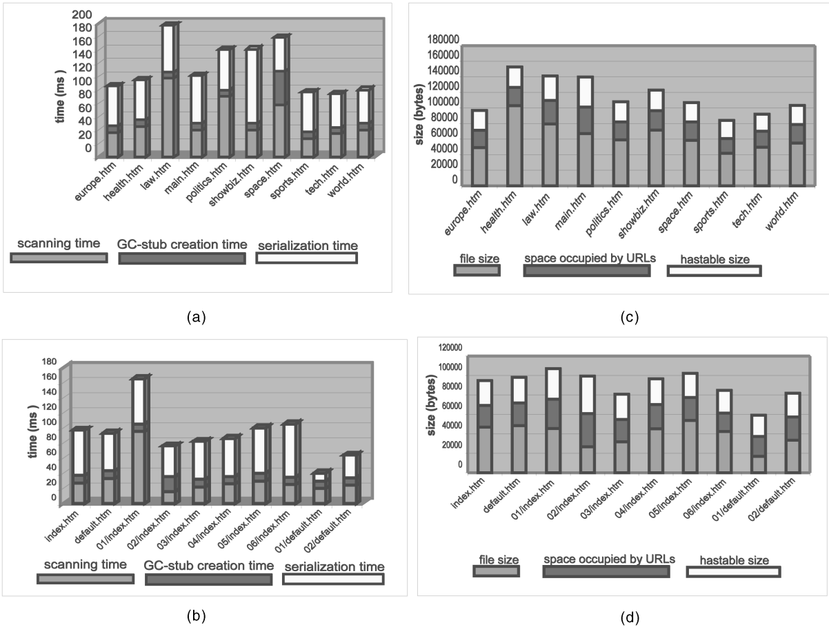
Fig. 8. Performance results for DGC. (a) Time spent for the top group, (b) time spent for the branch group, (c) space occupied for the top group, and (d) space occupied for the branch group.
