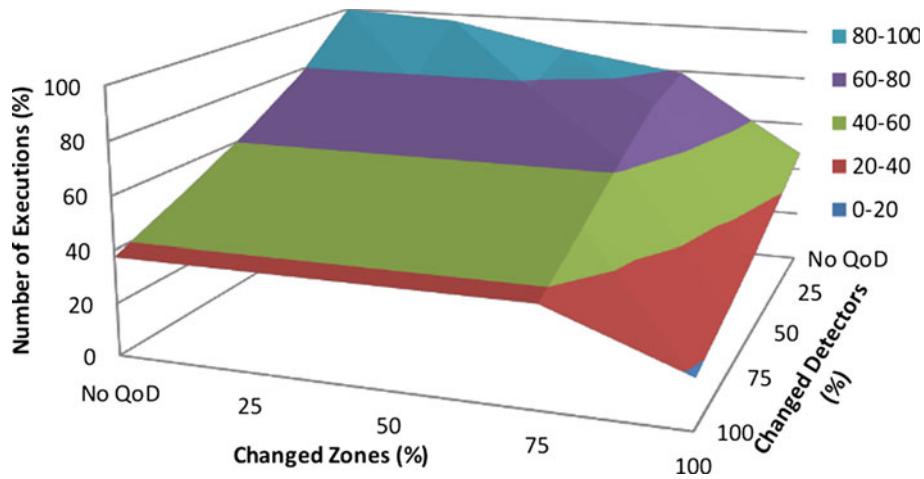
Figure 15 Hotspot executions.
