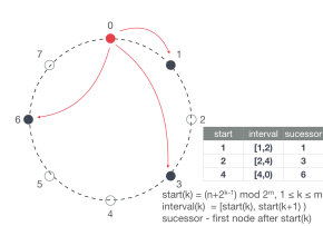
Fig. 12. Peer with ID=0 finger table
