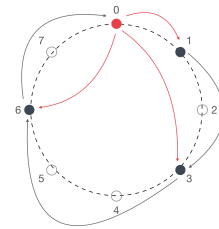
Fig. 11. Example of peer with ID = 0 fingers
