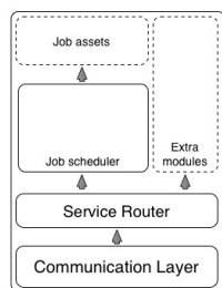
Fig. 13. Software layers at the peer level
