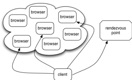
Fig. 1. browserCloud.js Overview
