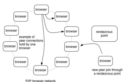
Fig. 2. browserCloud.js Distributed Architecture Overview
