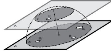
Figure 5: 3-dimensional VFC
