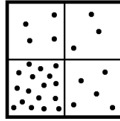
Figure 2: Region-based IM
