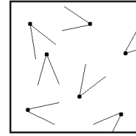
Figure 3: Visibility-based IM
