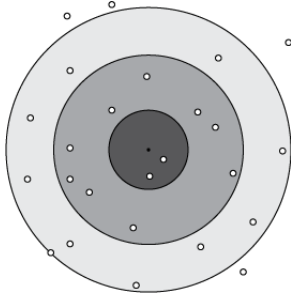
Figure 4: 2-dimensional VFC
