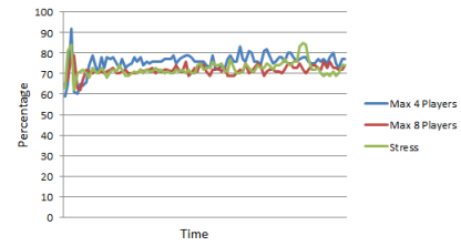
Figure 10: CPU consumption after VFC
