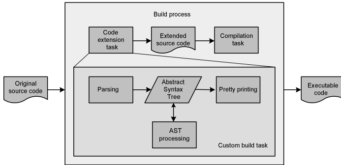
Fig. 1. Code generation flowchart
