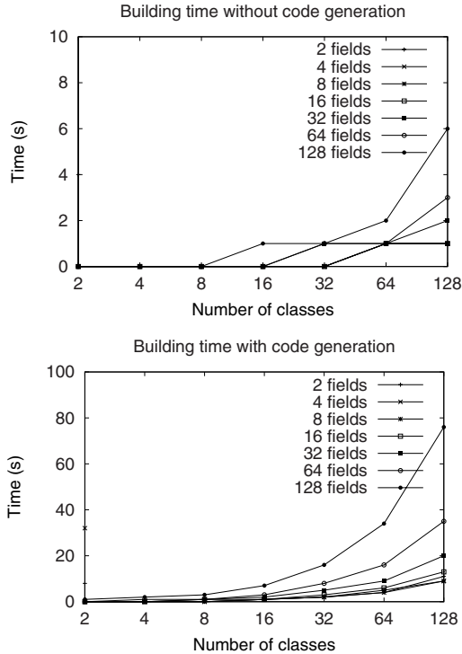
Fig. 2. Project building times with and without code generation
