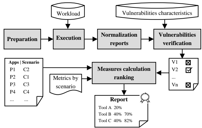
Fig. 5. Benchmarking procedure.
