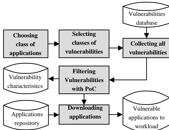
Fig. 3. Process for collecting vulnerable applications.
