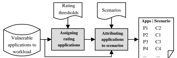
Fig. 4. Process for assigning applications to scenarios.
