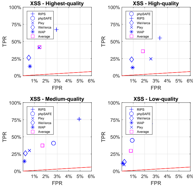
Fig. 7. Benchmark XSS comparison by scenario.
