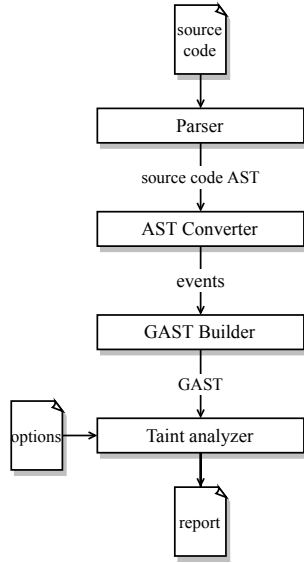
Fig. 1. The GT tool data flow and architecture
