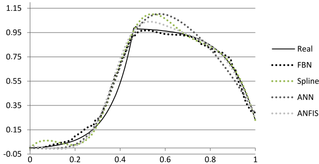
Fig. 4. Correlation results.
