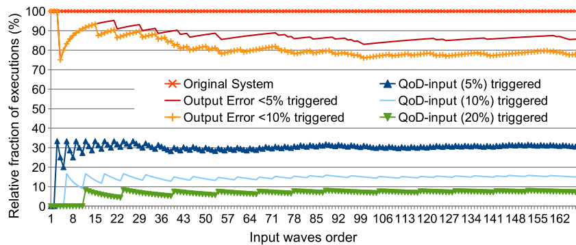
Fig. 12. Resource usage.
